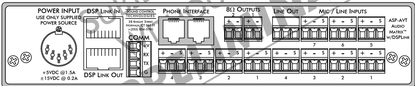
Series II ASP-AVT Audio Matrix w/Telephone Interface & 2-Channel Power Amplifier Rear Panel
