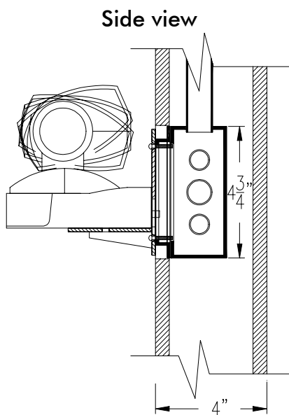
Camera wall-mount bracket
