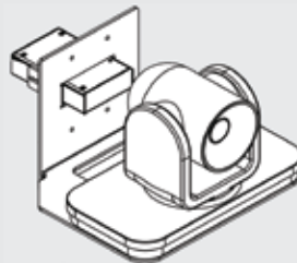
RC2-RK2 Rack Shelf
