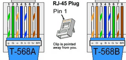
Integrator supplied Single CAT5e or CAT6 UTP Cable 300' Maximum EIA568A or B
